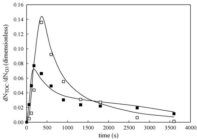
Fig. 7. Evolution of the moles of carbon mineralized by unit mole of ozone in runs with wastewater samples taken in April (□) and June (■). The symbols correspond to experimental values with derivatives obtained by a numerical non-model-based procedure.
