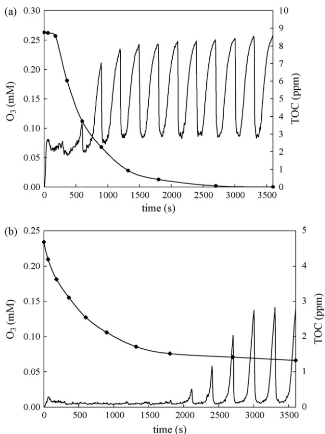
Fig. 2. Evolution of TOC (●) and concentration of dissolved ozone during the treatment of wastewater with repeated injections of 0.15 mL of H 2 O 2 (30%, w/v) every 300 s. Samples taken (a) in April and (b) in September.
