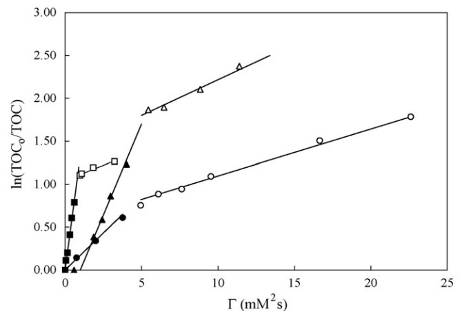
Fig. 4. Logarithmic decay of TOC for representative runs corresponding to April (triangles), June (circles) and July (squares) as a function of \Gamma defined in Eq. (9). Filled and empty symbols indicate the two TOC decay periods at which data were fitted.
