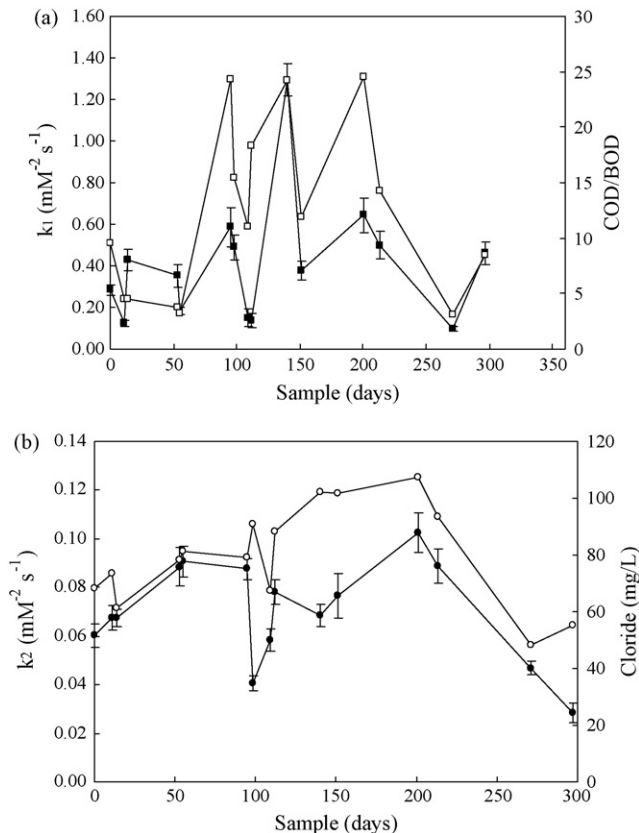
Fig. 5. Dependence of reaction kinetic parameters for TOC decay during the first (a) and second (b) fitting period. Filled symbols correspond to k_1 and k_2 . Also shown COD/BOD (□) and chloride (○) in wastewater samples.
