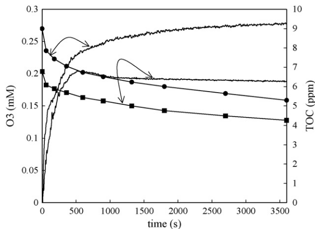
Fig. 3. Evolution of TOC and concentration of dissolved ozone during the ozonation treatment of wastewater without injection of hydrogen peroxide for samples taken in April (●) and in June (■).
