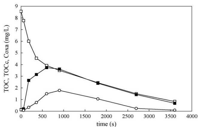
Fig. 6. Evolution of experimental TOC (□) and TOC calculated from the concentration of acids formic, acetic and oxalic (■). Empty circles represent the concentration of oxalic acid. In this run, the transition from first to second kinetic period took place at 360 s.
